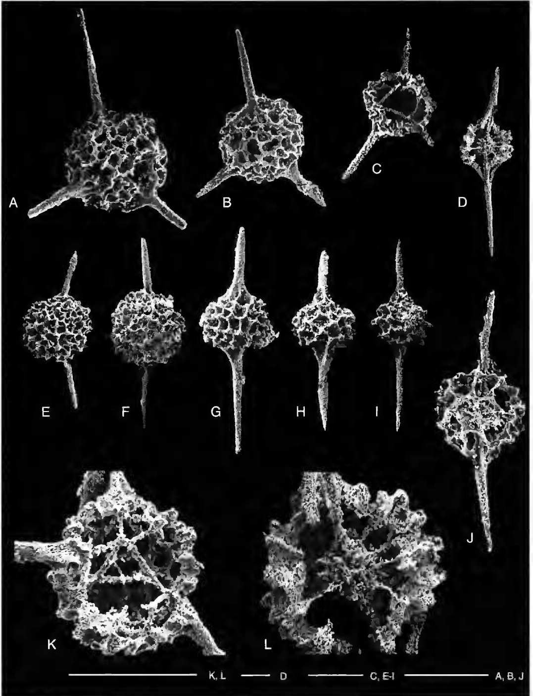
FIG. 11. — A-C, K, Cryptostephanidium longispinosum (Sashida). A, DEUY-YK3625; B, DEUY-YK3634; C, showing arch-like skeleton of aj, DEUY-YK3641; K, showing internal structure of A, L, D, and V spinules, DEUY-YK3633; D, G-J, L, Pantanellium (?) virgeum Sashida; D, DEUY-YK3474; G, DEUY-YK3614; H, DEUY-YK3649; I, DEUY-YK3438; J, DEUY-YK3498; L, enlargement of D showing cortical shell and beams, DEUY-YK3475; E, F, Pantanellium (?) sp. A; E, DEUY-YK3466; F, DEUY-YK3430. Scale bars: 100 \mu m.
